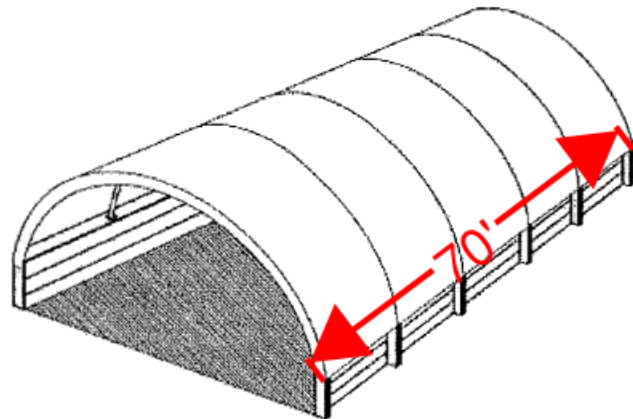
30' WALL MOUNT - COMMON BAY
