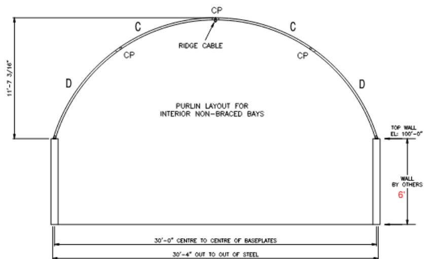
30' WALL MOUNT - COMMON BAY
