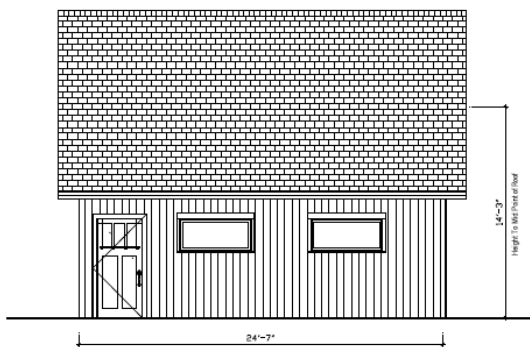
EAST ELEVATION
