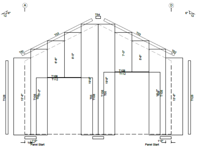
ENDWALL SHEETING & TRIM: FRAME LINE 1 PANELS: 26 Ga. AWR - Need Color
