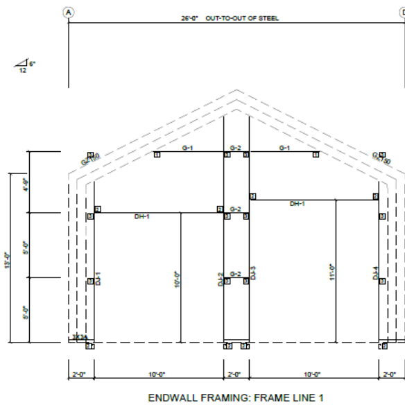
ENDWALL FRAMING: FRAME LINE 1
